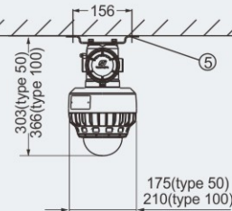
X: ceiling type
